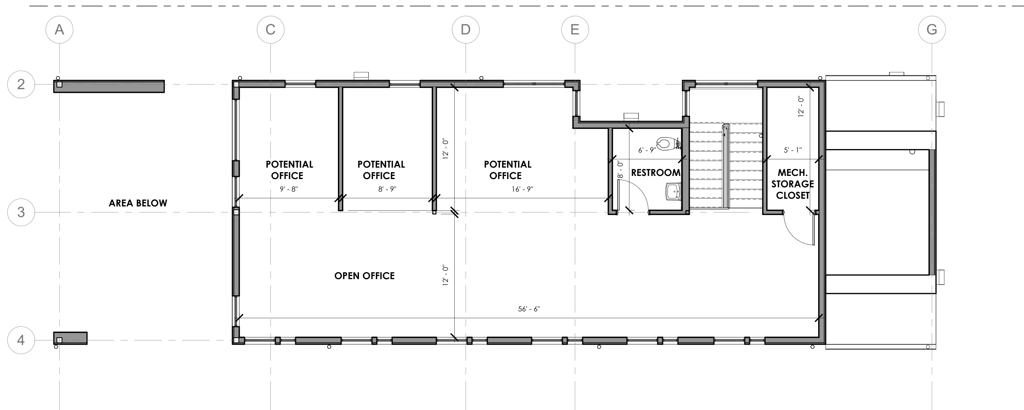
2 second floor 3/16" = 1'-0"
