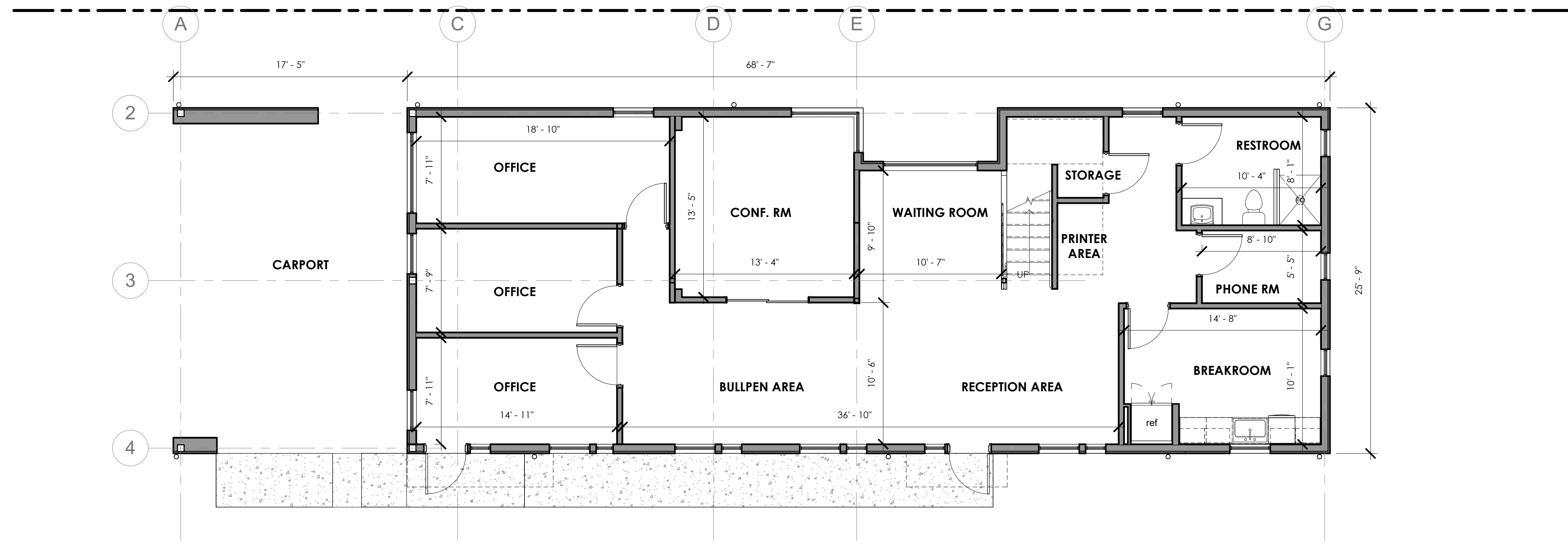
1 first floor 3/16" = 1'-0"
