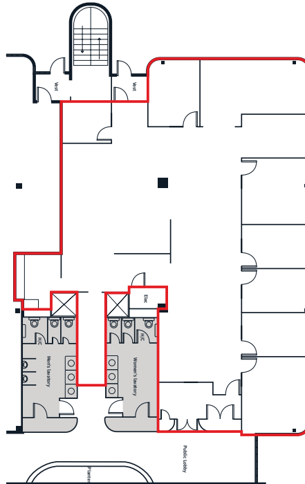
One Corporate Drive 1st floor: 5,088 SF
