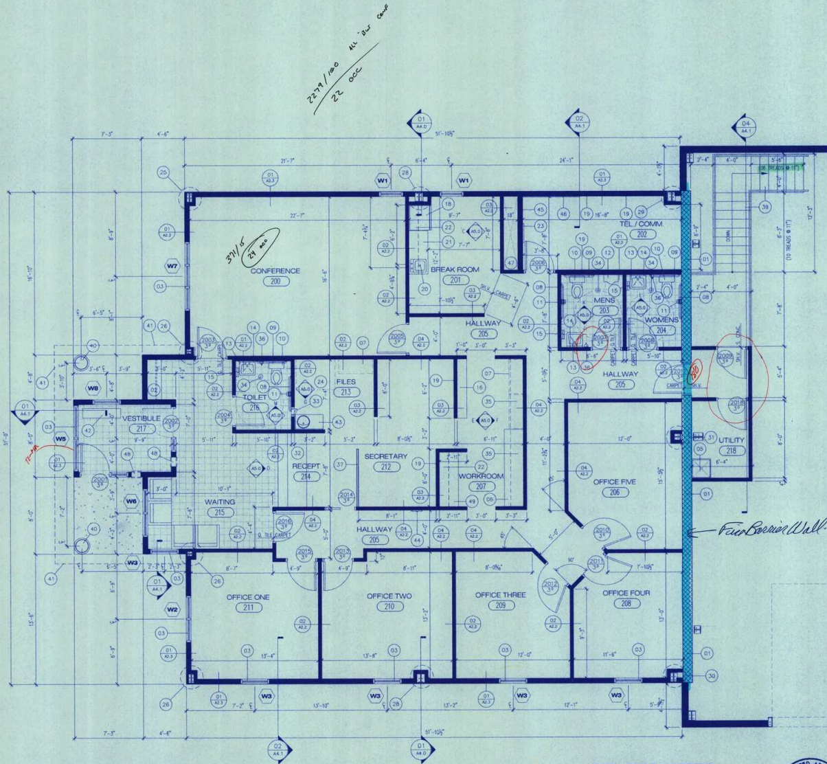
1 ENLARGED SECOND FLOOR OFFICE PLAN SCALE: 1/4" = 1'-0"
