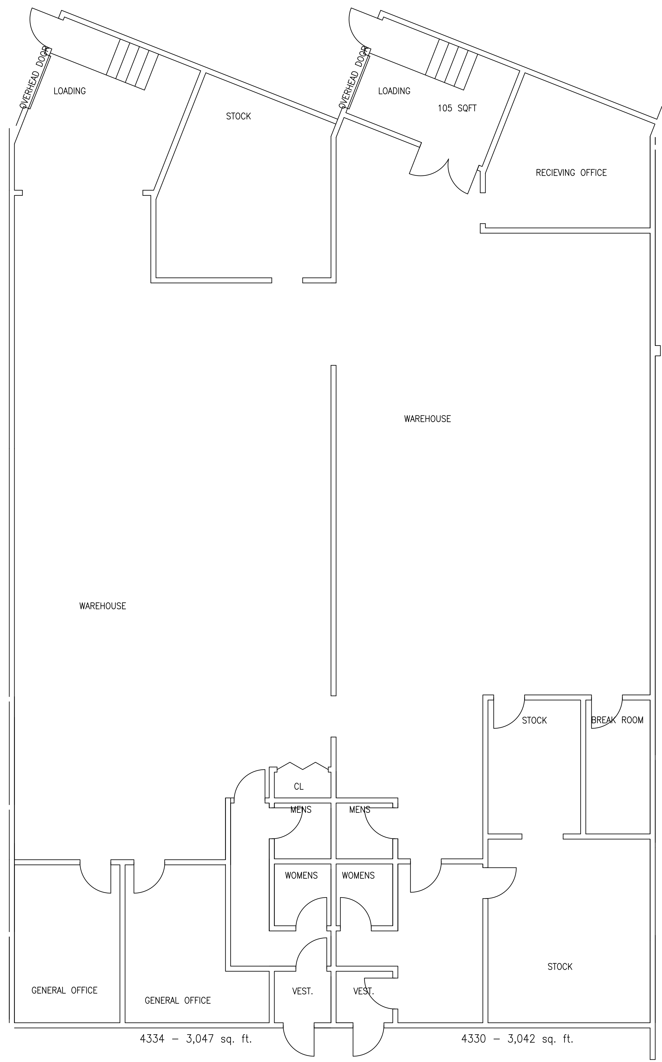
1 Unit 4330 & 4334 - Floor Plan 3/16" = 1'-0" 0 5' 10' NORTH
