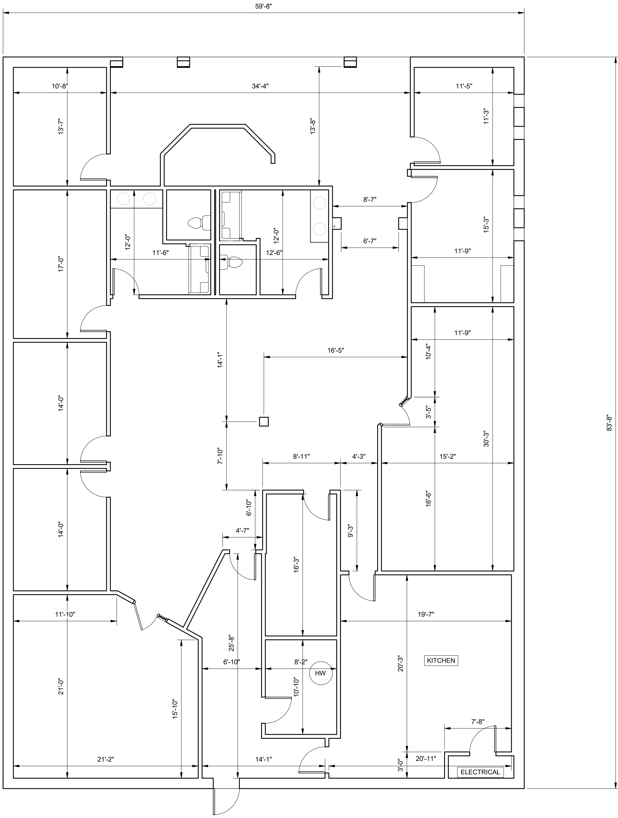
1 PLAN SCALE: 3/16" = 1'-0"
