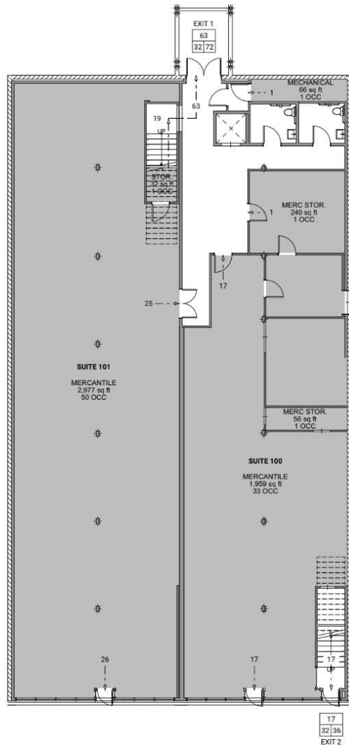
1ST FLOOR CODE PLAN
