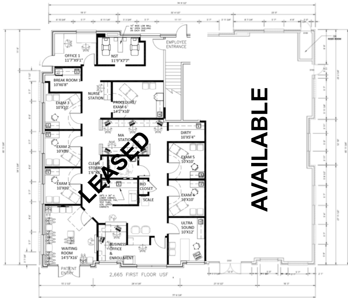
1 GROUND FLOOR PLAN - EXISTING SCALE: 3/16"=1'
