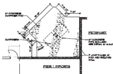
2 DUMPSTER PAD PLAN SCALE: 1/4" = 1'-0"
