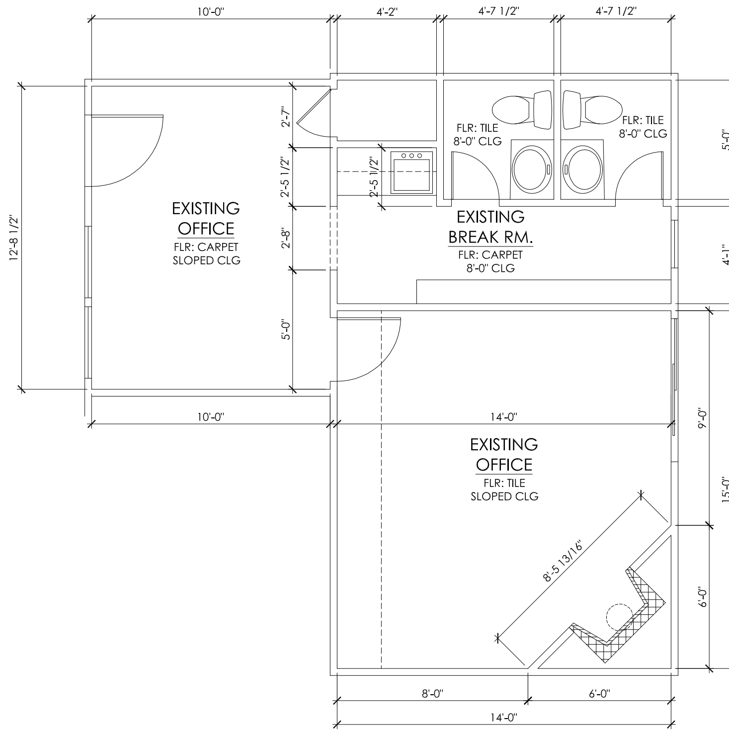
EXISTING FLOOR PLAN SCALE 1/4" = 1'-0"
