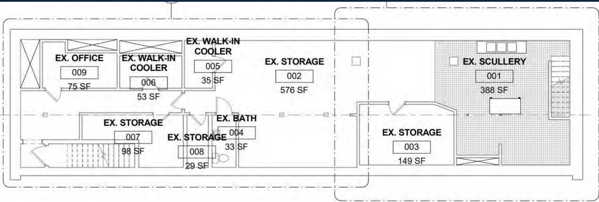
① BASEMENT PLAN 1/8" = 1'-0"
