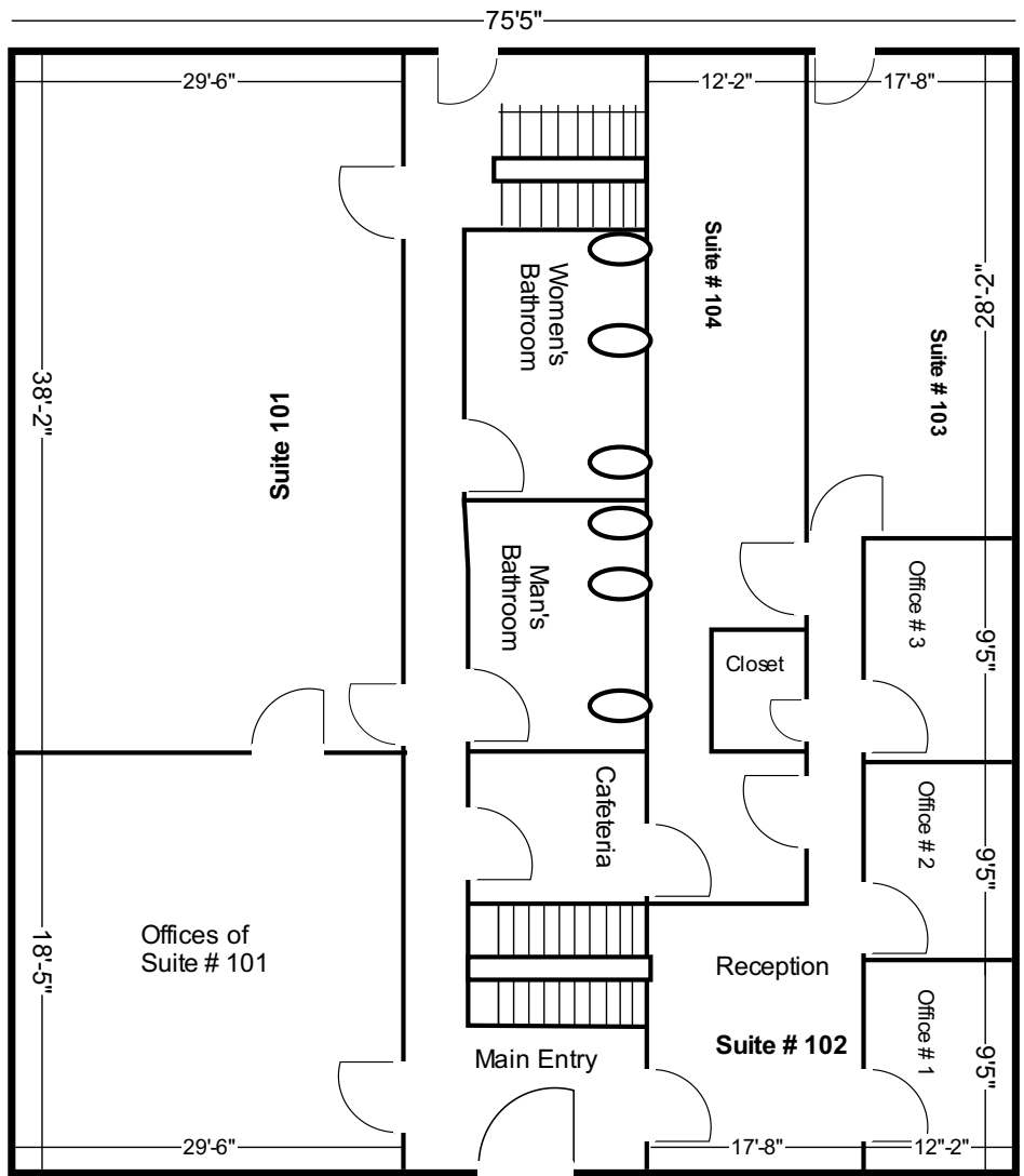
Existing Floor Plan of 1st Floor 4139 Gardendale St. San Antonio, TX 78229
