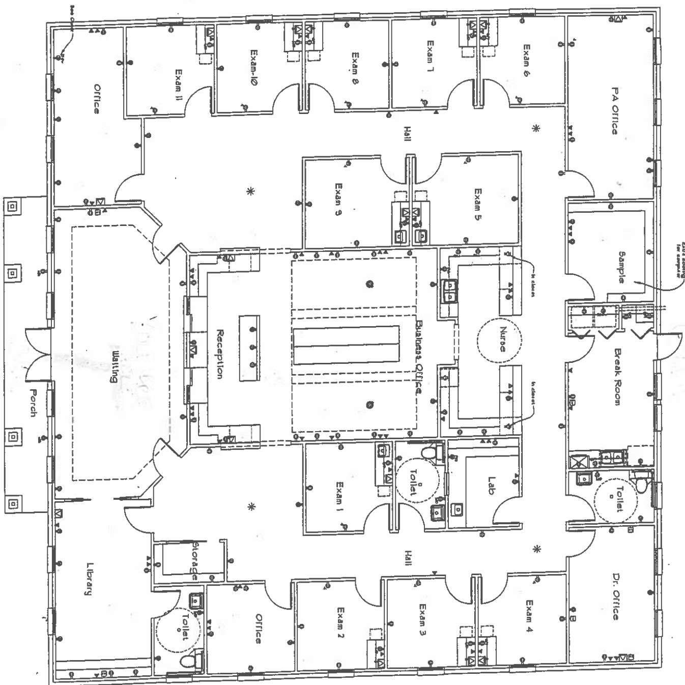
ELECTRICAL FLOOR PLAN 1/17/70
