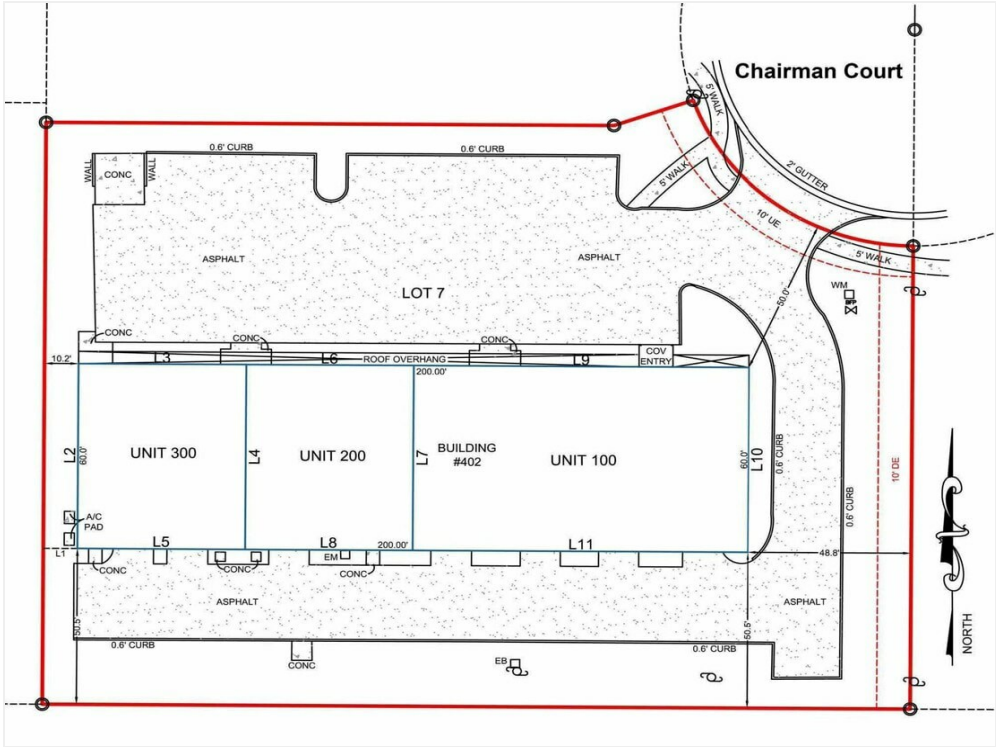
402 chairman property survey
