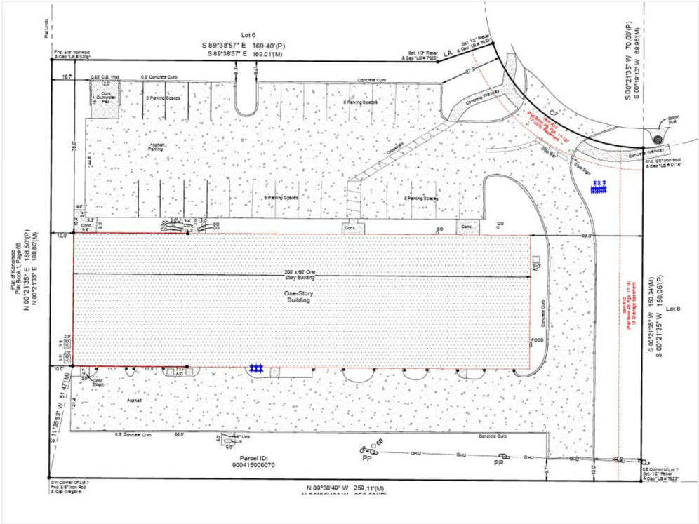
402 chairman property survey with parking lot
