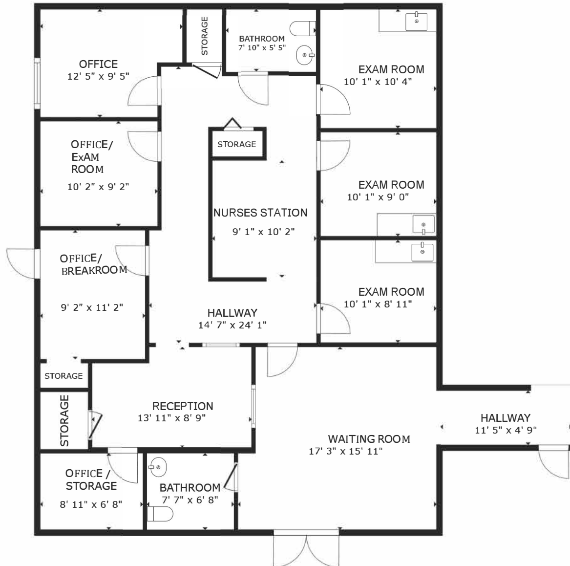
FLOOR PLAN
