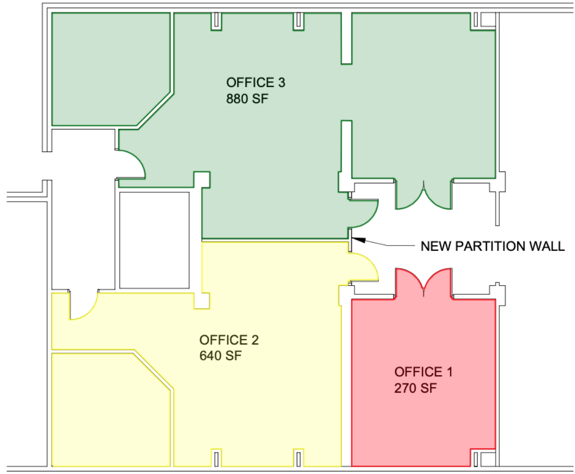
PRELIMINARY SPACE DIVISION - FLOOR PLAN SCALE: 1/8"=1'-0"
