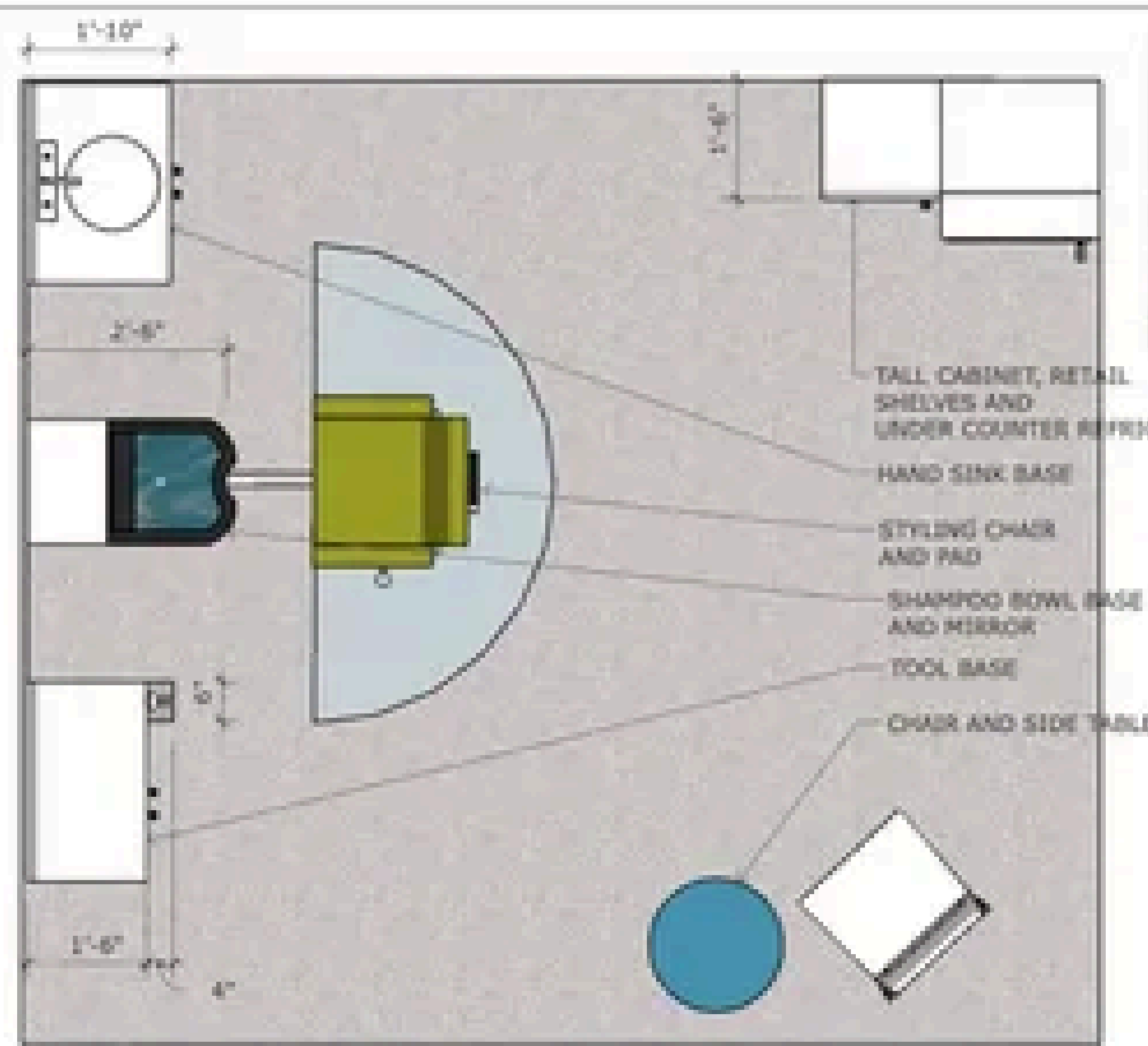
2 Salon Suite Plan 1/2" = 1'-0"
