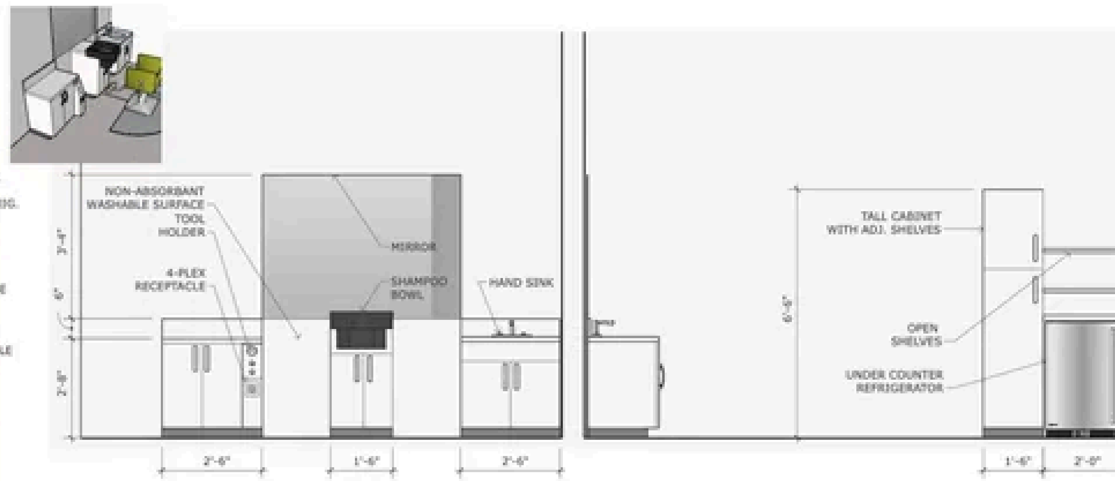
3 Salon Suite Cabinetry Elevation 1/2" = 1'-0"
