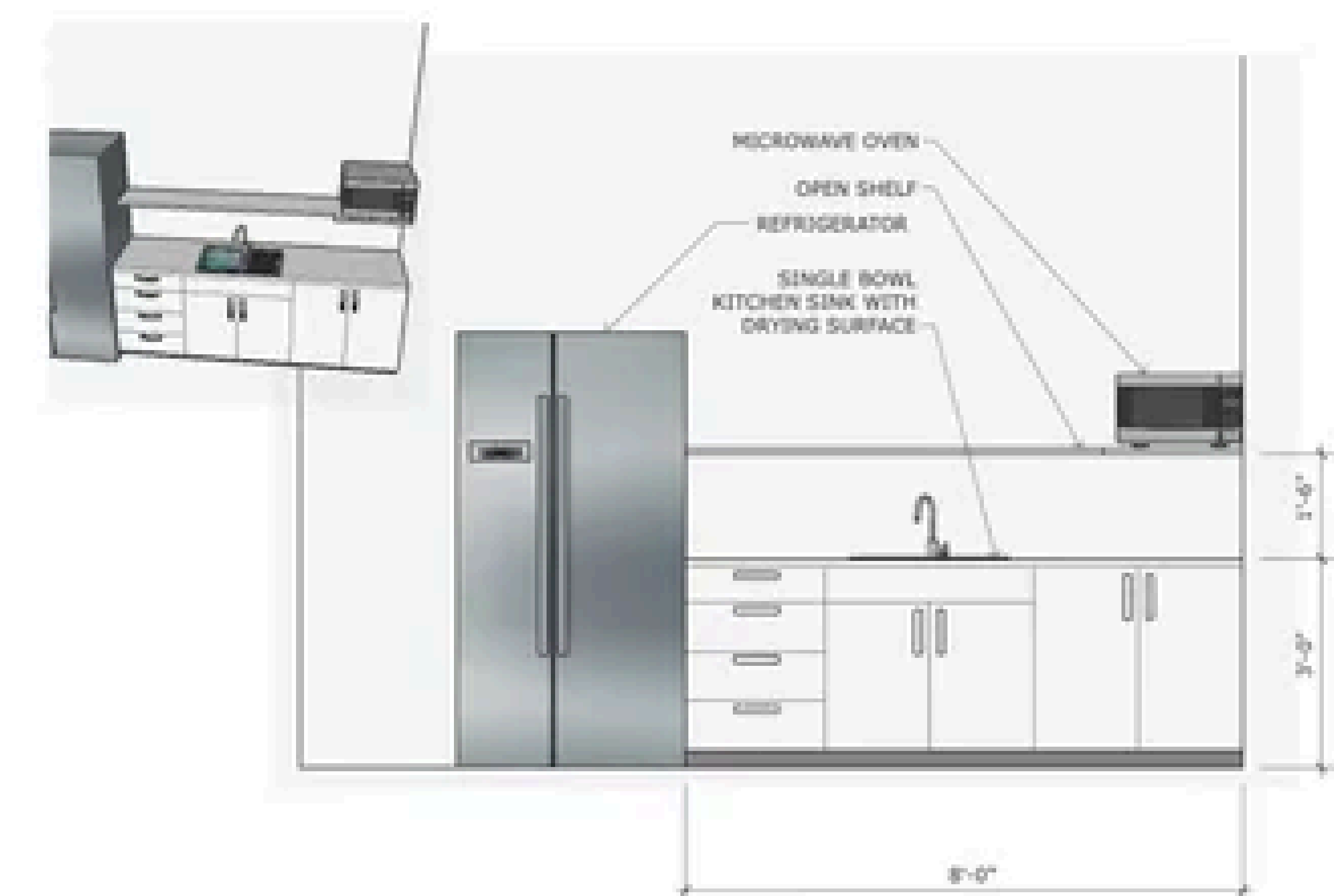
4 Utility Room Cabinetry Elevation 1/2" = 1'-0"
