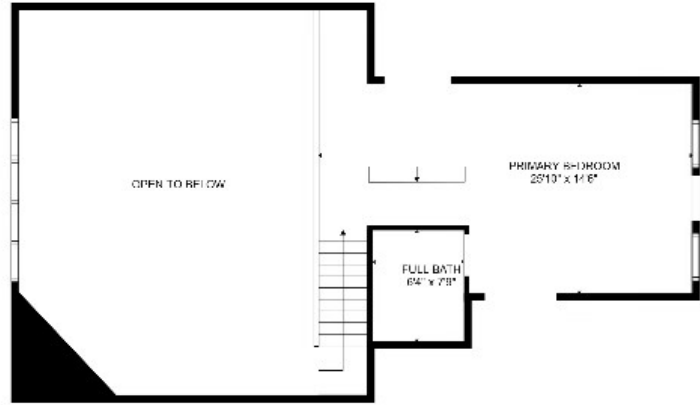
FLOOR 3
