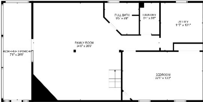
FLOOR 1
