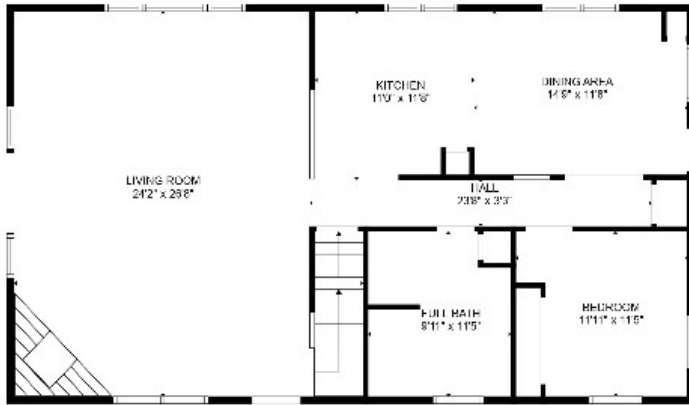
FLOOR 2
