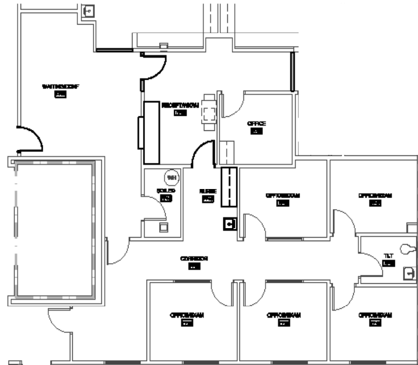
TEST-FIT LAYOUT
