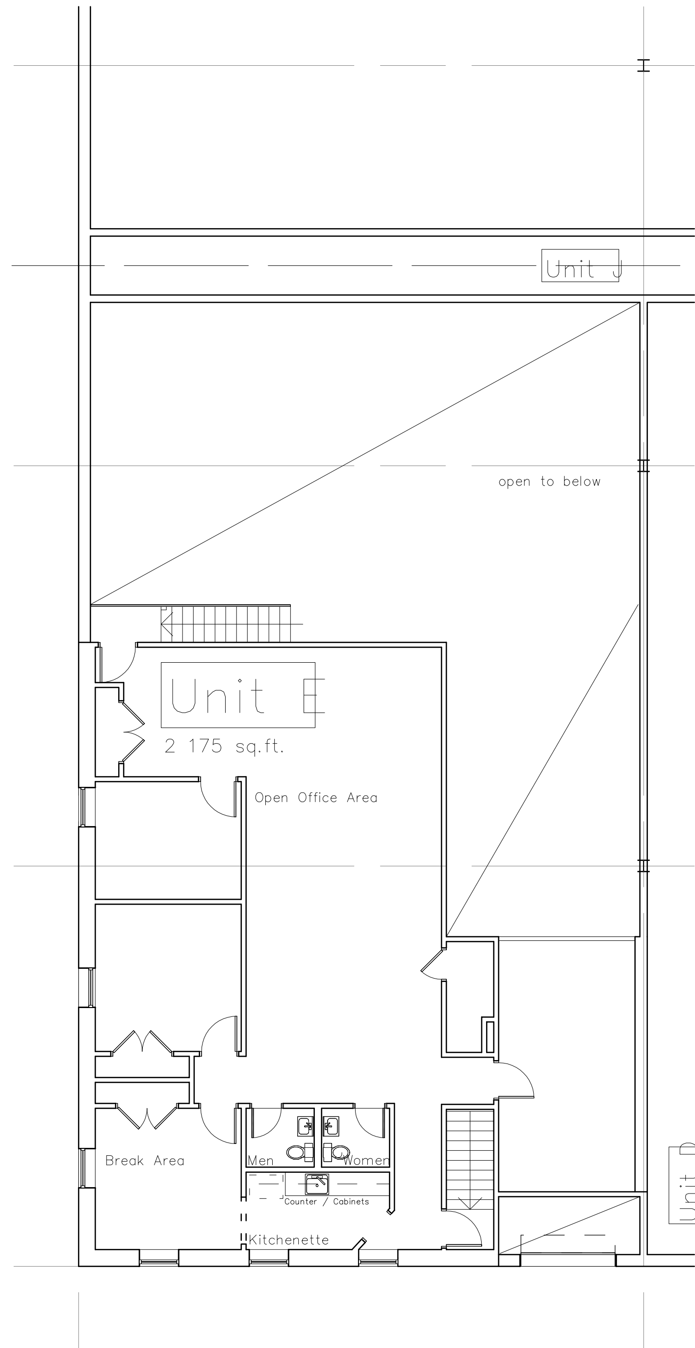
Mezzanine Plan
