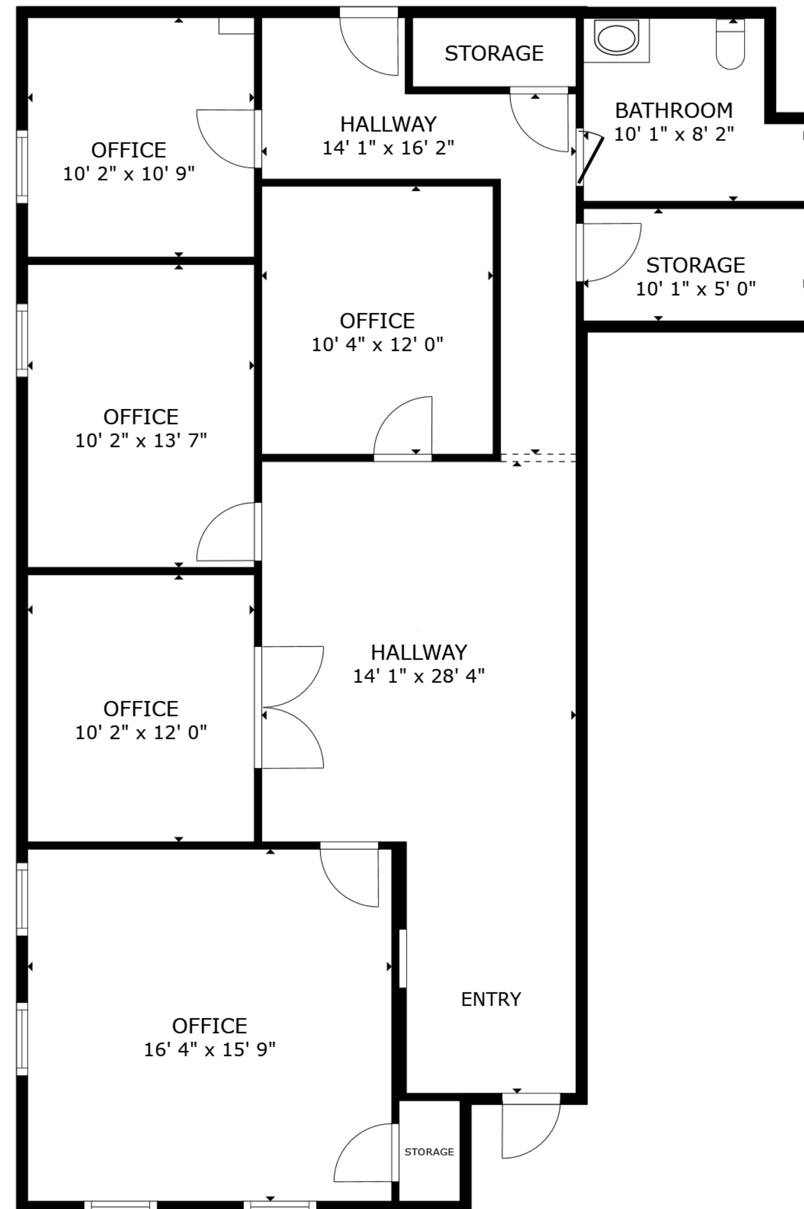
FLOOR PLAN
