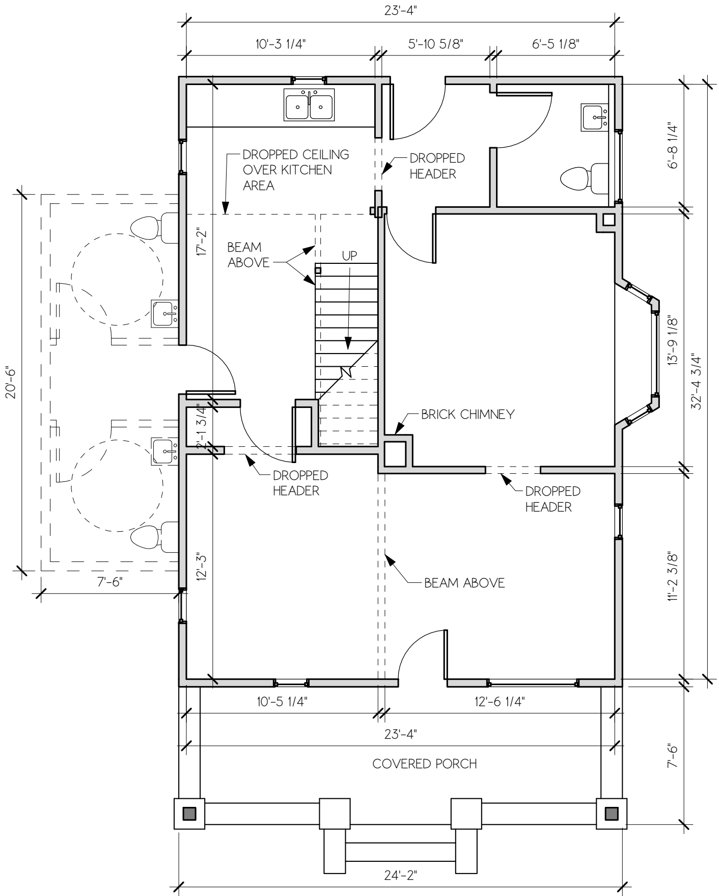
1 FIRST FLOOR EXISTING PLAN SCALE: 3/16" = 1'-0"
