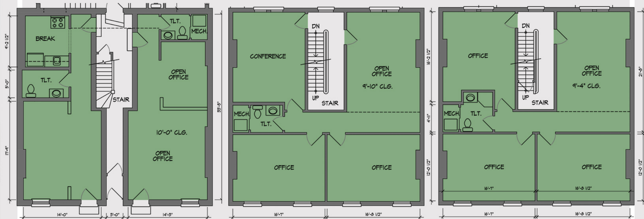
2nd Floor 1,000 SF
