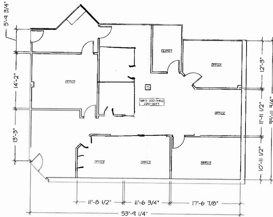
F A-2.1 SUITE 200 SCALE: 3/32" = 1'-0" 2,295 SF
