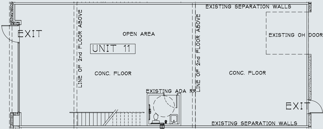
MAIN LEVEL FLOOR PLAN SCALE: 1/8"=1'-0"
