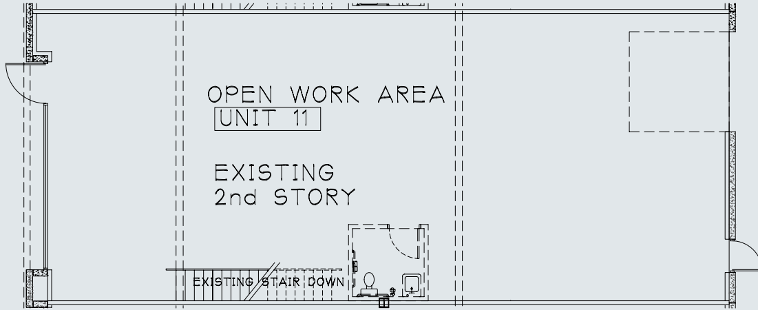
SECOND STORY FLOOR PLAN SCALE: 1/8"=1'-0"
