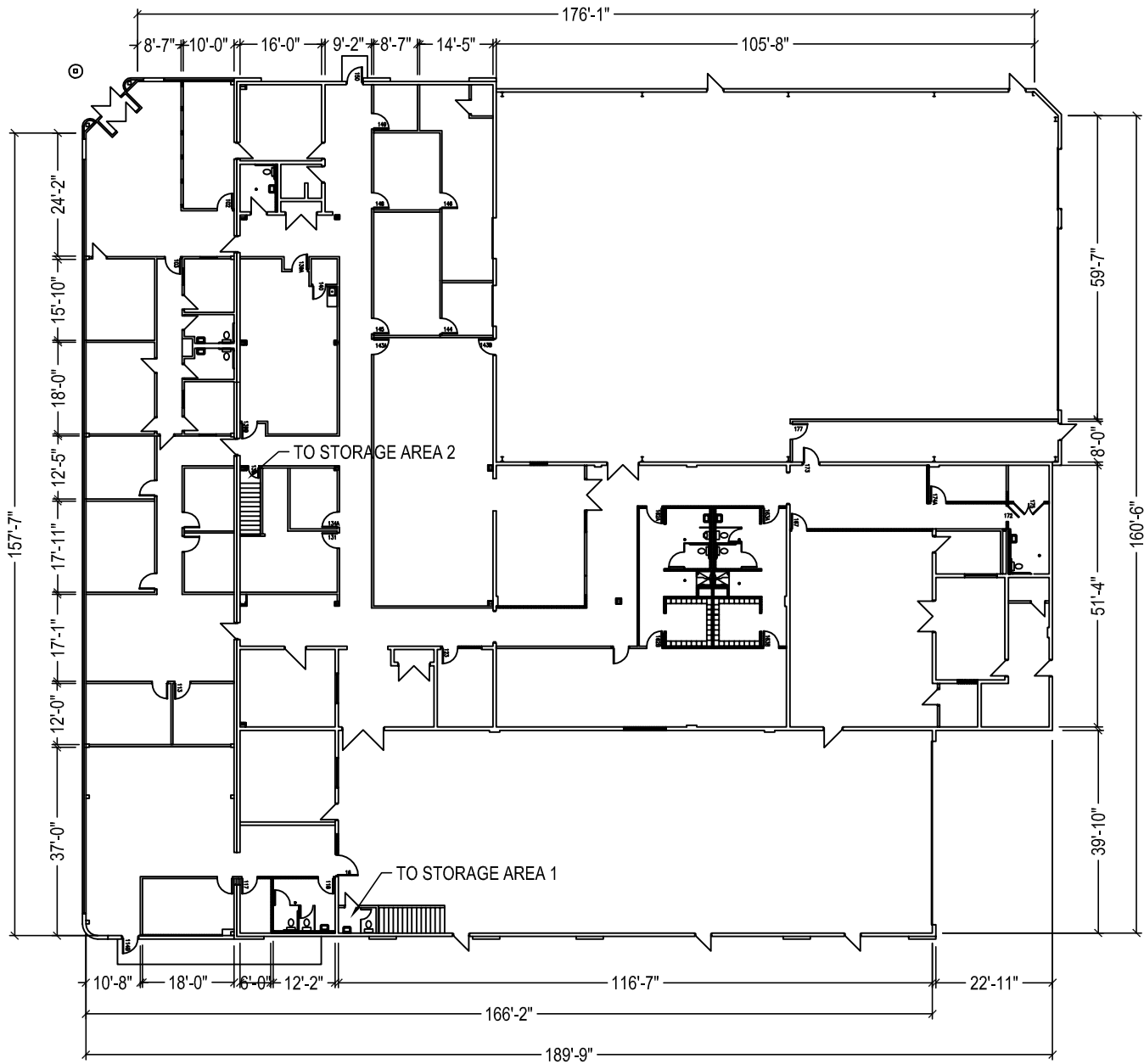
FLOOR PLAN SCALE: 1/32"=1'-0"
