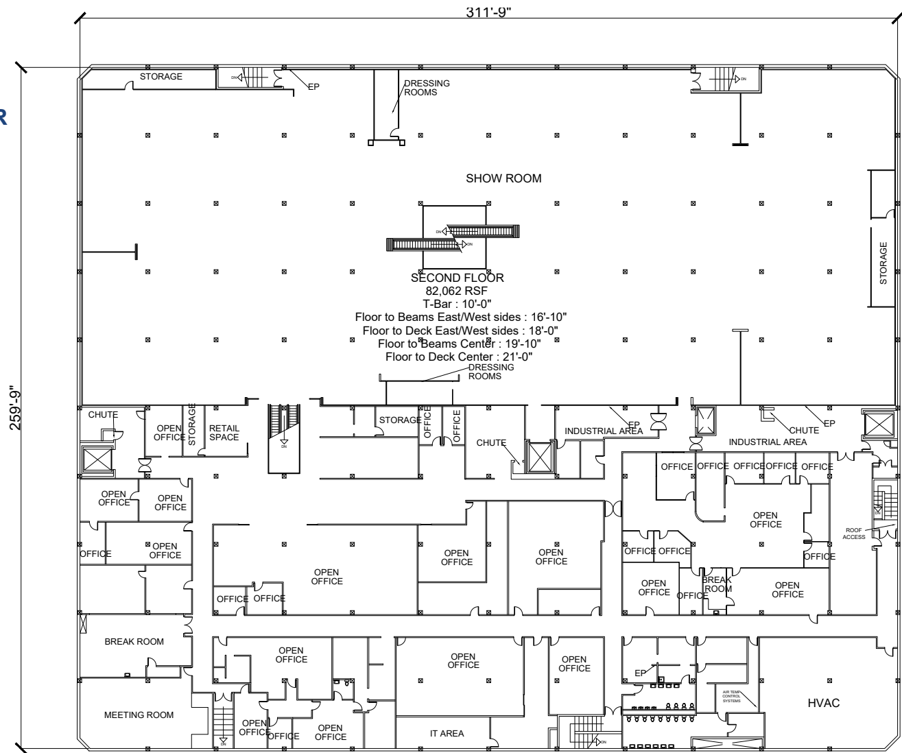
FLOOR PLAN SECOND FLOOR
