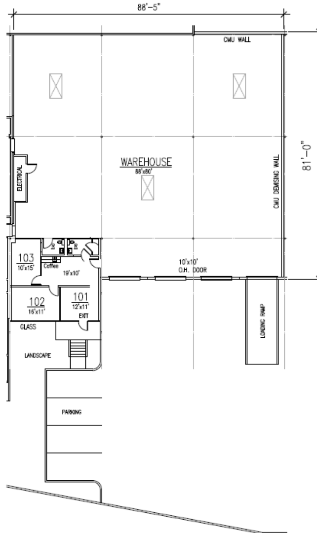
4585 FLOOR PLAN
