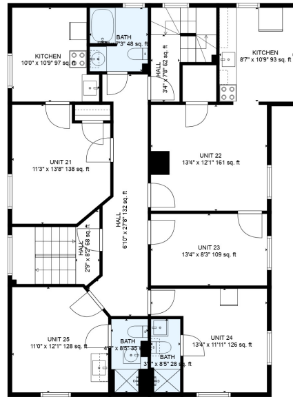
FLOOR 2
