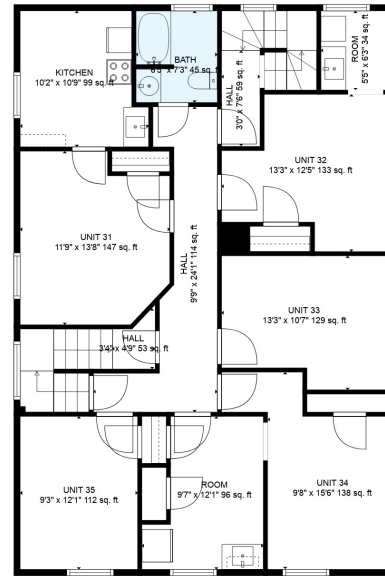
FLOOR 3
