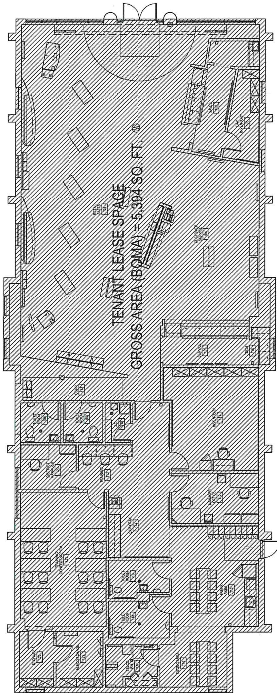
PLAN NORTH FLOOR PLAN - EXISTING 3/32" = 1'-0"
