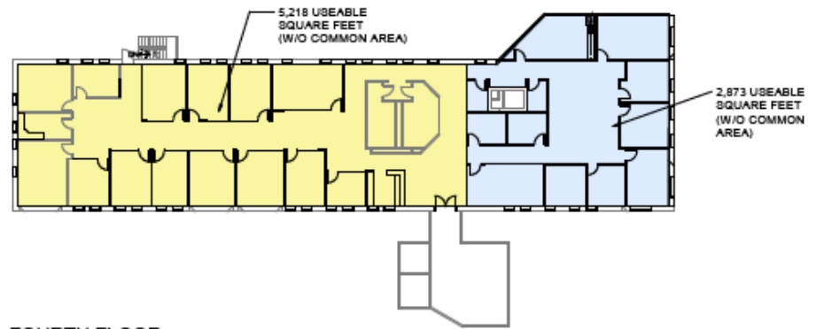
④ FOURTH FLOOR 1/16" = 1'-0"
