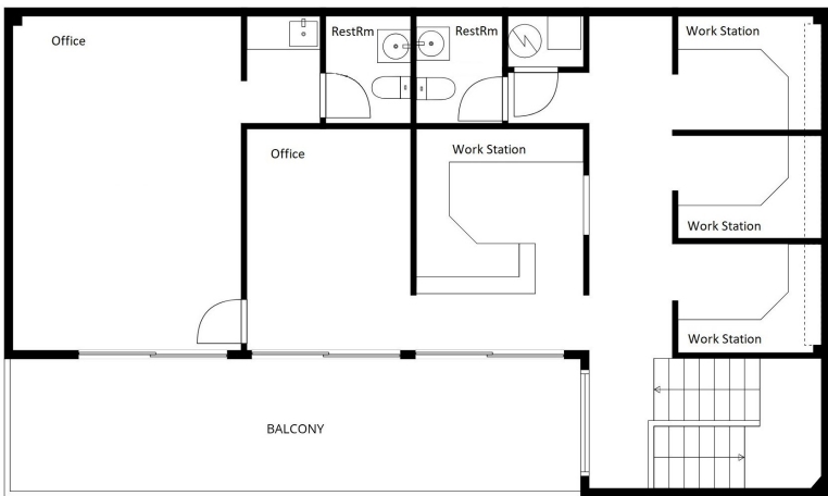
FLOOR 2
