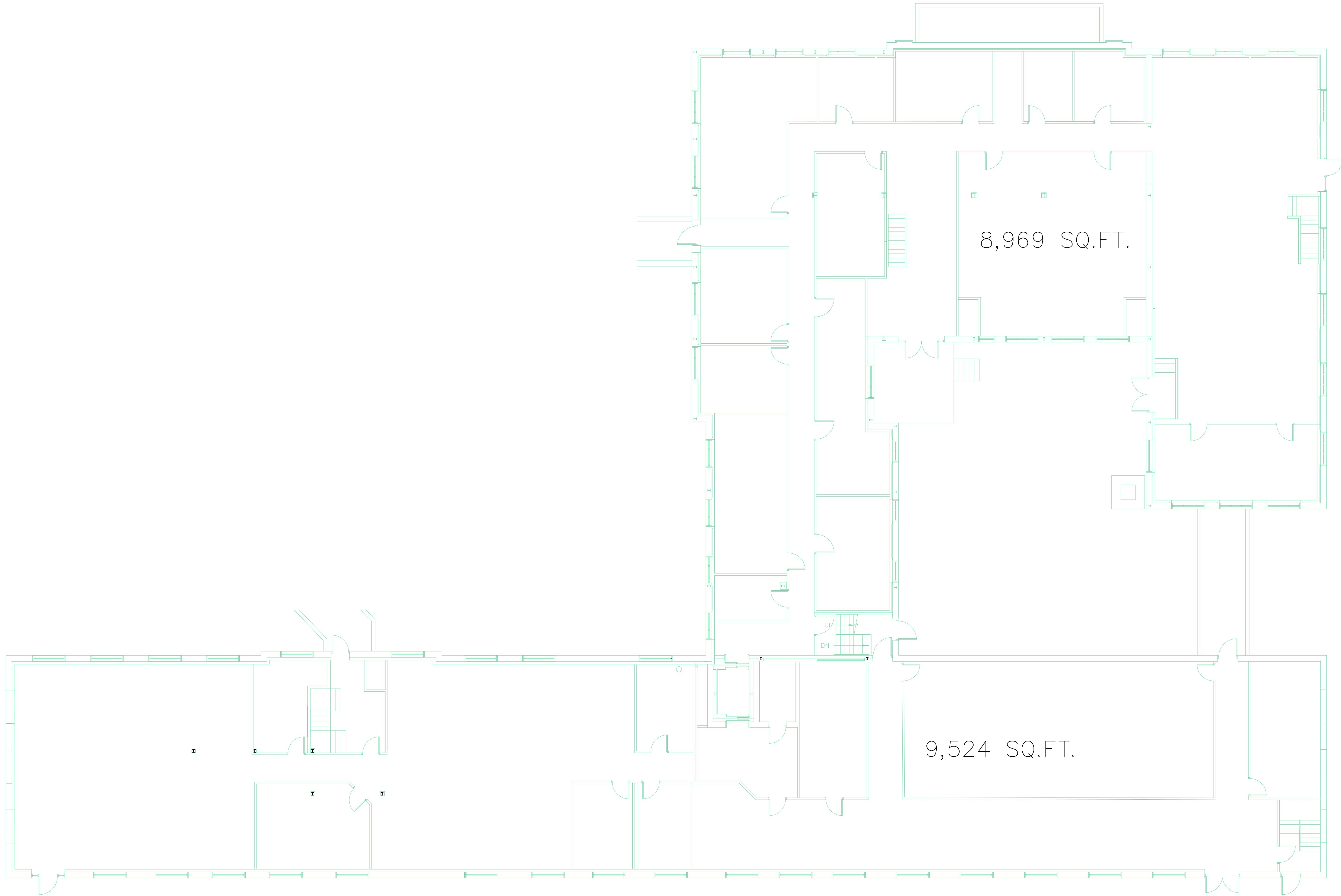
LOWER LEVEL PLAN SCALE: 1/8"=1'-0"
