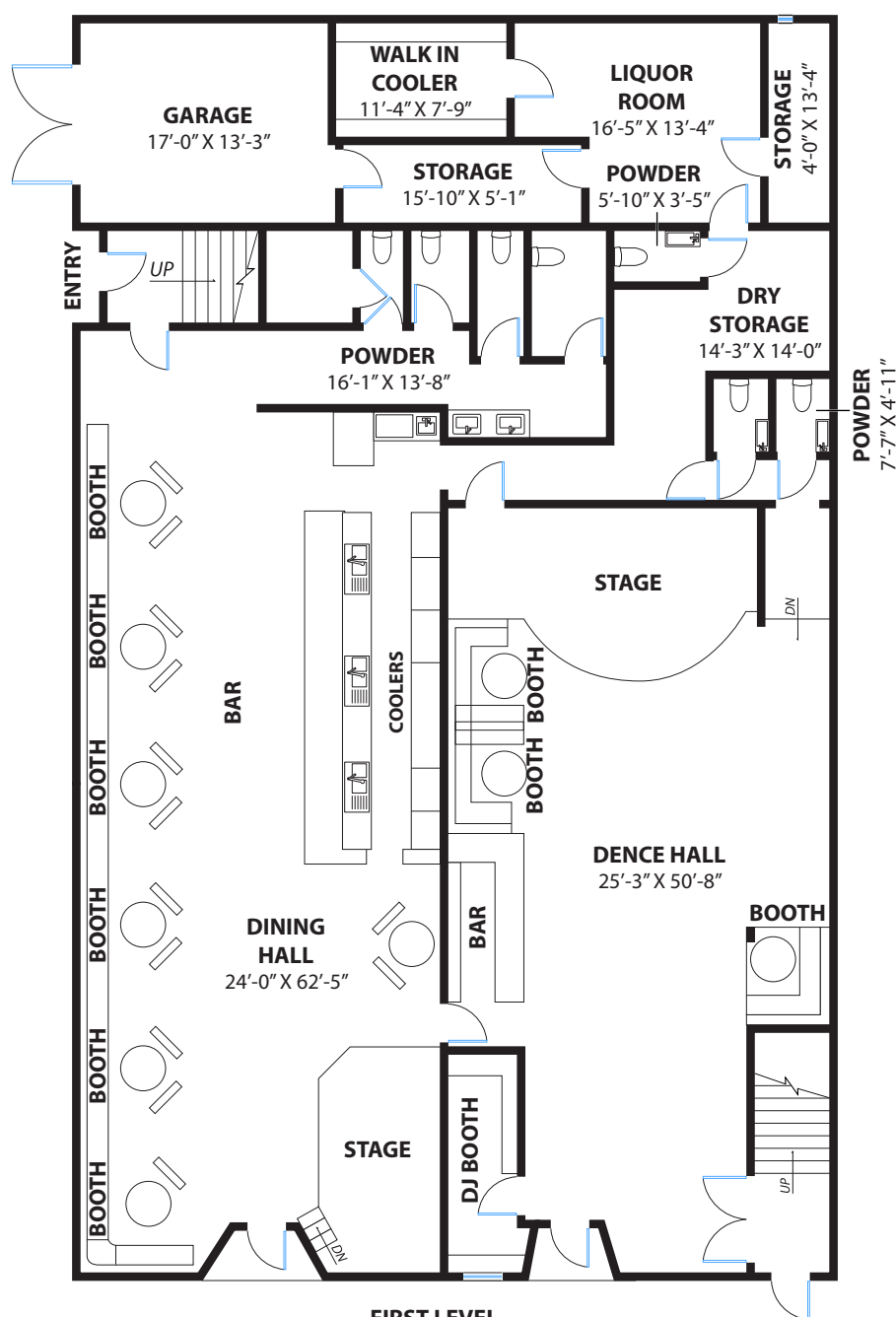
FIRST LEVEL
