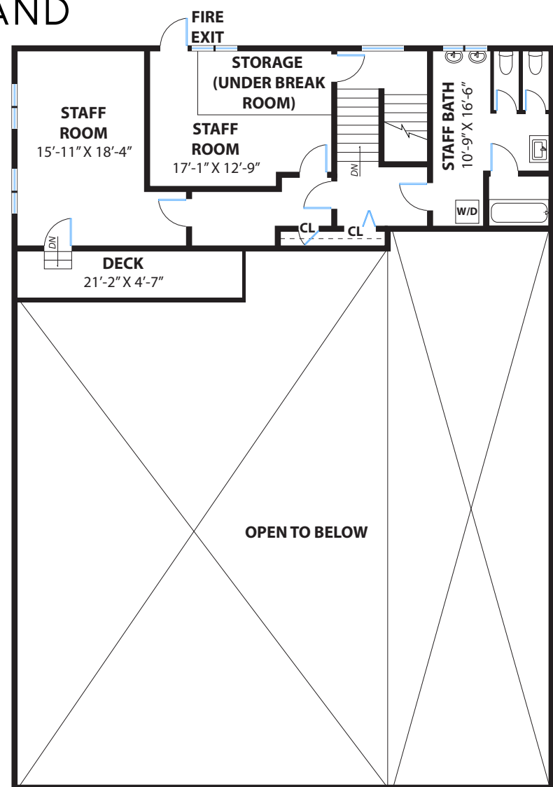
THIRD LEVEL
