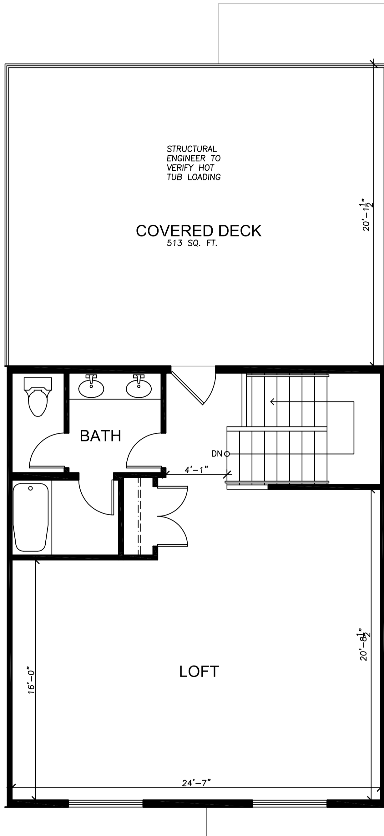
QUAIL HOLLOW 4-BEDROOM 3RD FLOOR PLAN 3/24/2022
