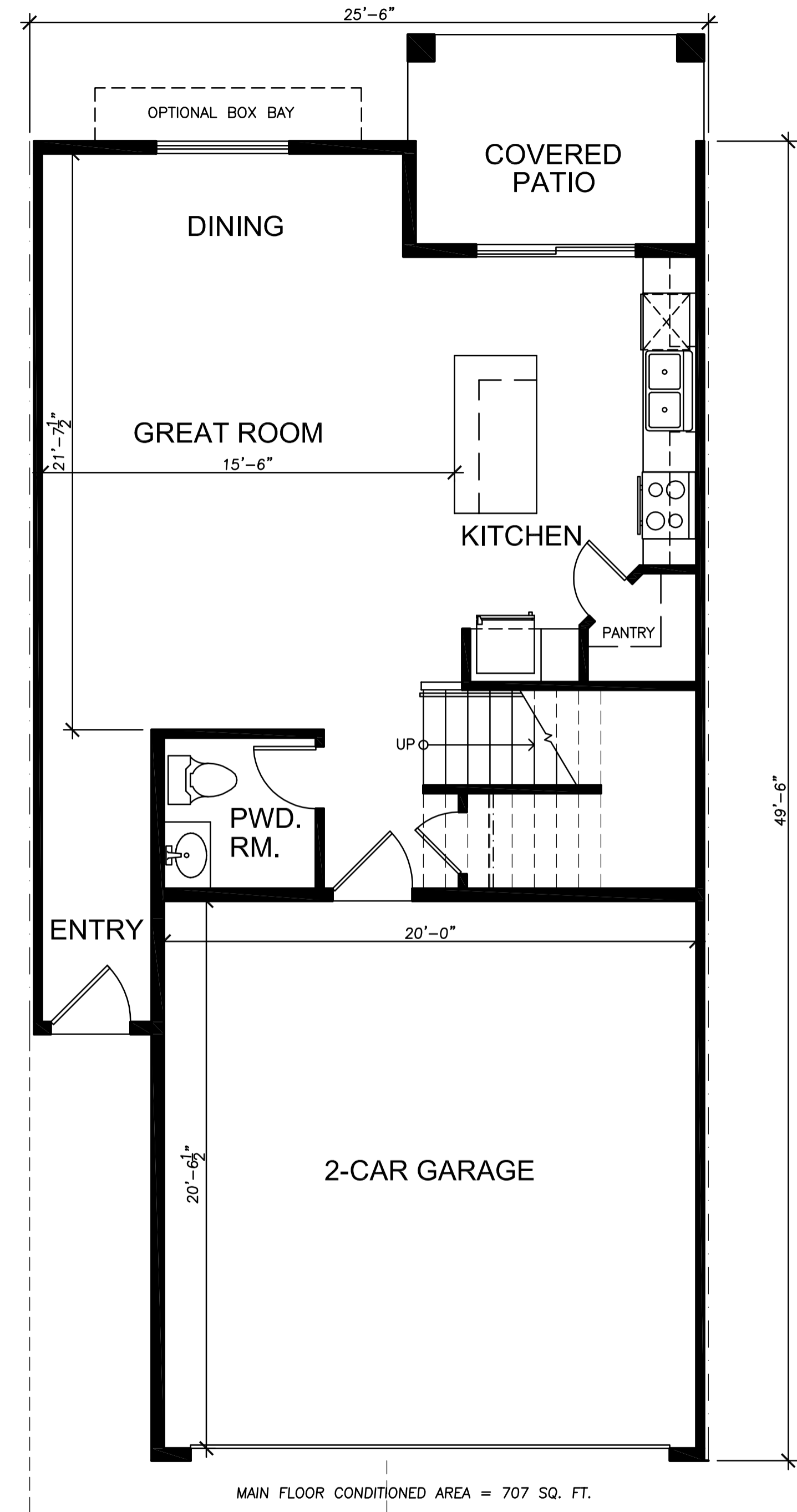
QUAIL HOLLOW MAIN FLOOR PLAN OPT. 2.c 3/22/2022
