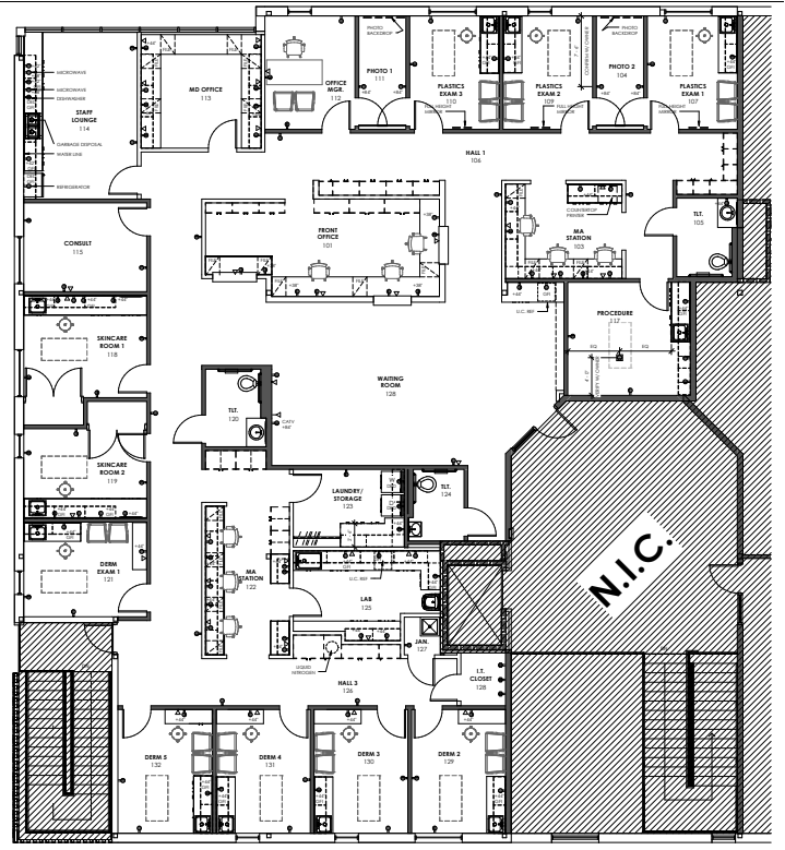
FURNITURE PLAN
