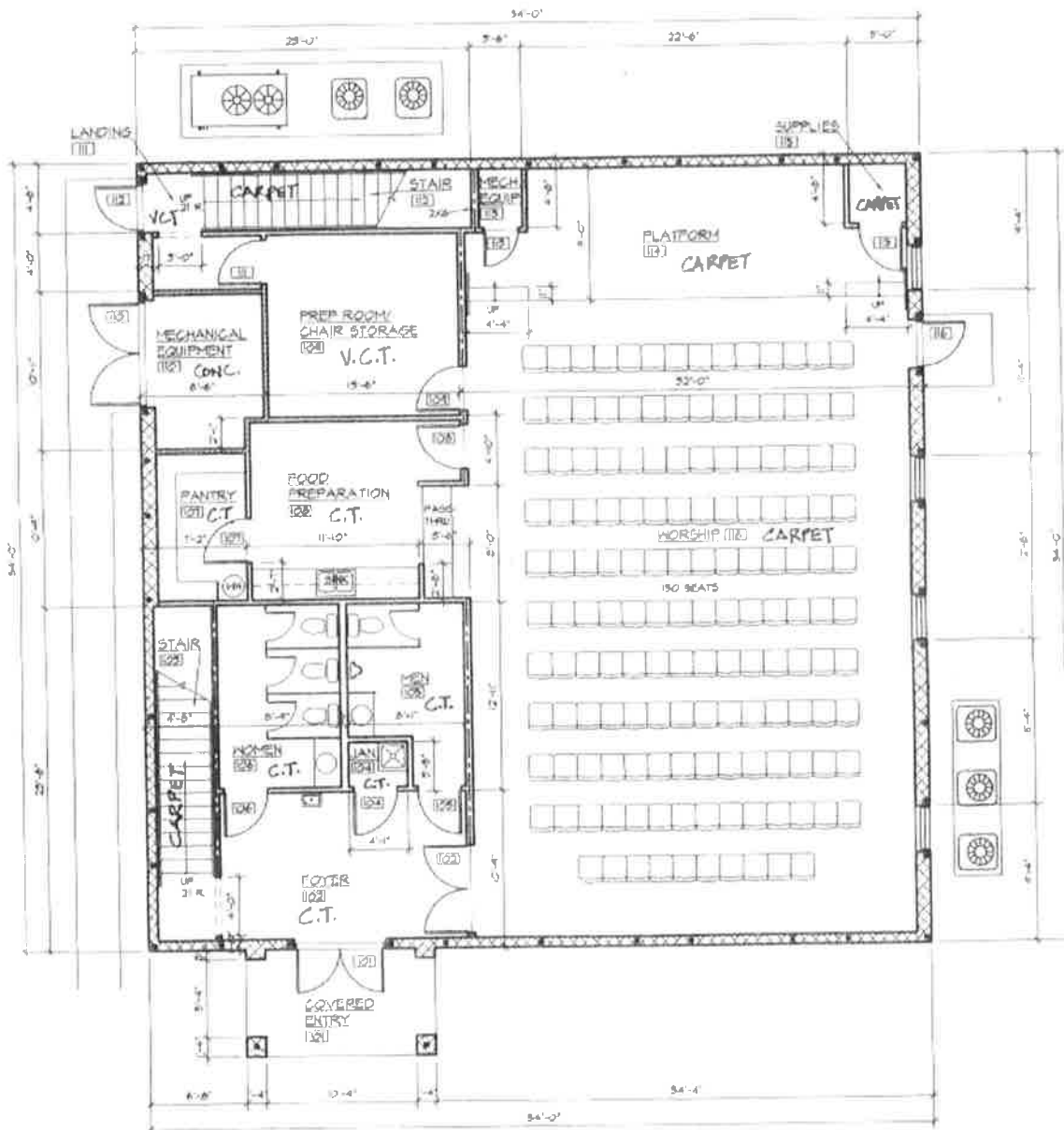
FIRST FLOOR PLAN SCALE: 3/16" = 1'-0" 2,96 SQ FT
