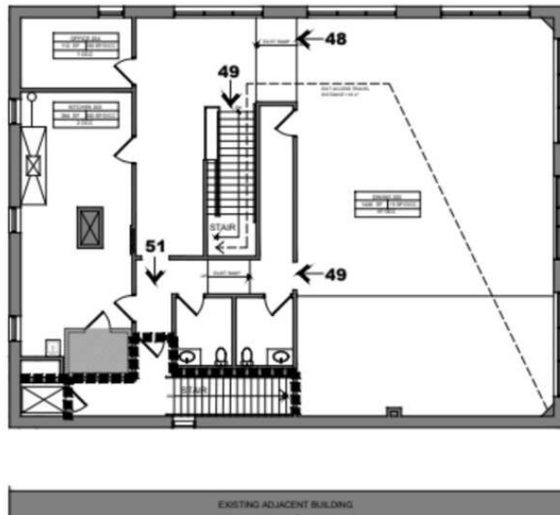
3 SECOND FLOOR CODE PLAN SCALE: 1/8" = 1'-0"
