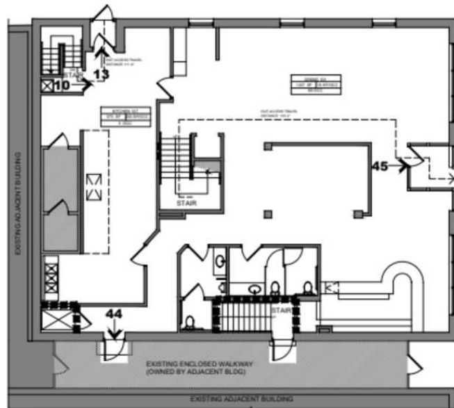
2 FIRST FLOOR CODE PLAN SCALE: 1/8" = 1'-0"
