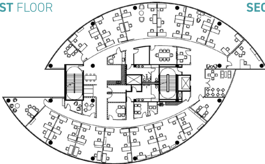
THIRD FLOOR
