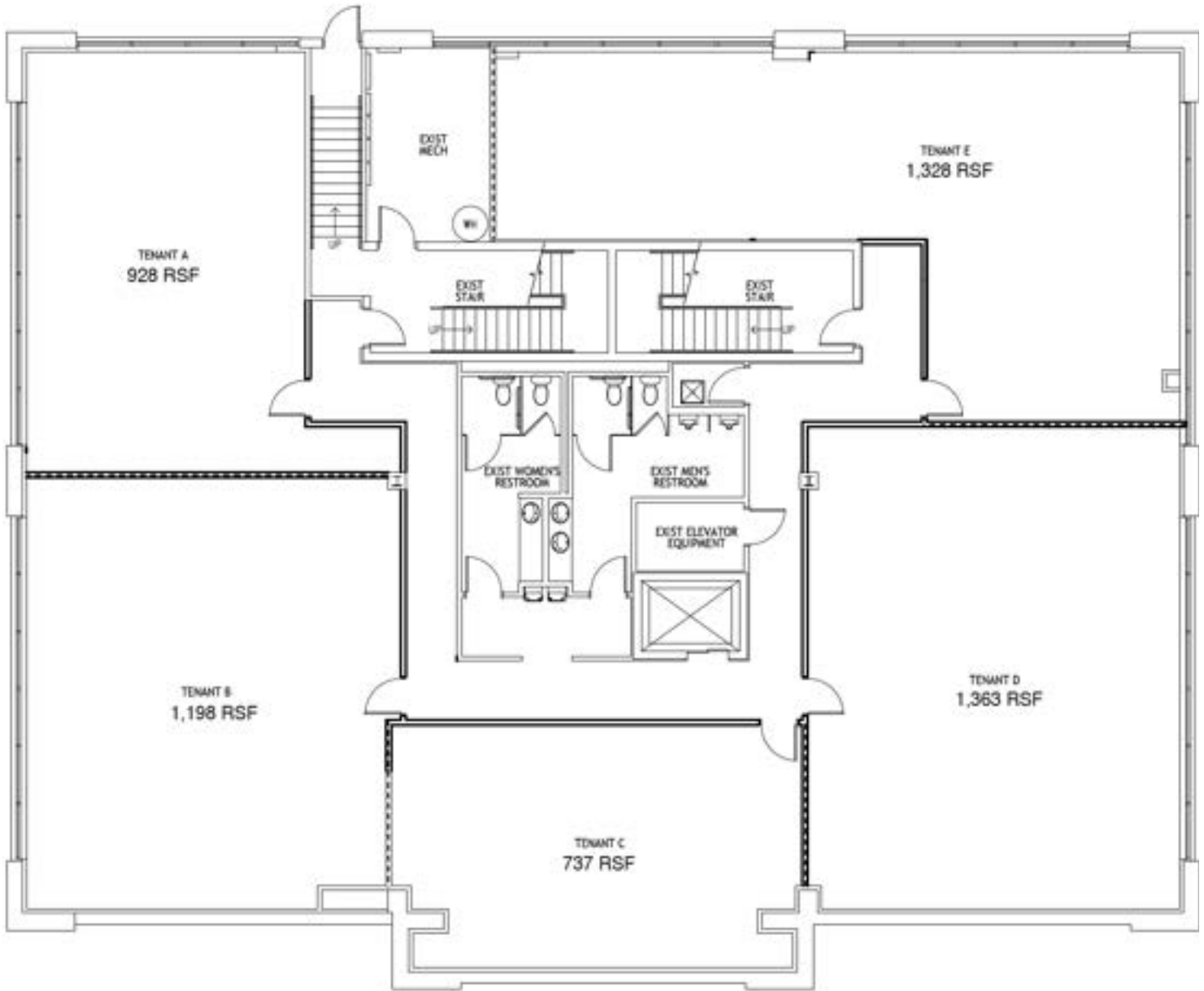
LOWER LEVEL FLOOR PLAN 1/8" = 1'-0" 0' 2' 4' 8' 12'
