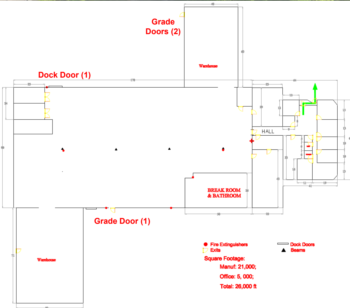
Floor Plan
