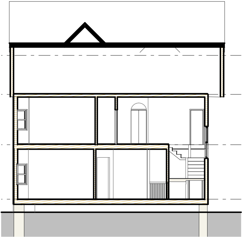
B2 Building Section 3/32" = 1'-0"
