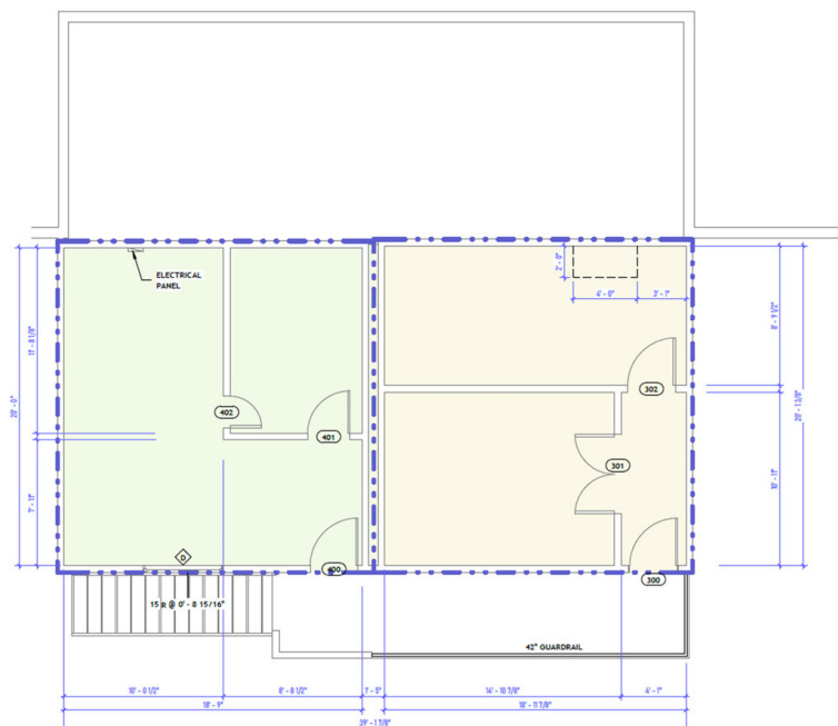
② SECOND FLOOR PLAN - OPTION 3 1/4" = 1'-0"
