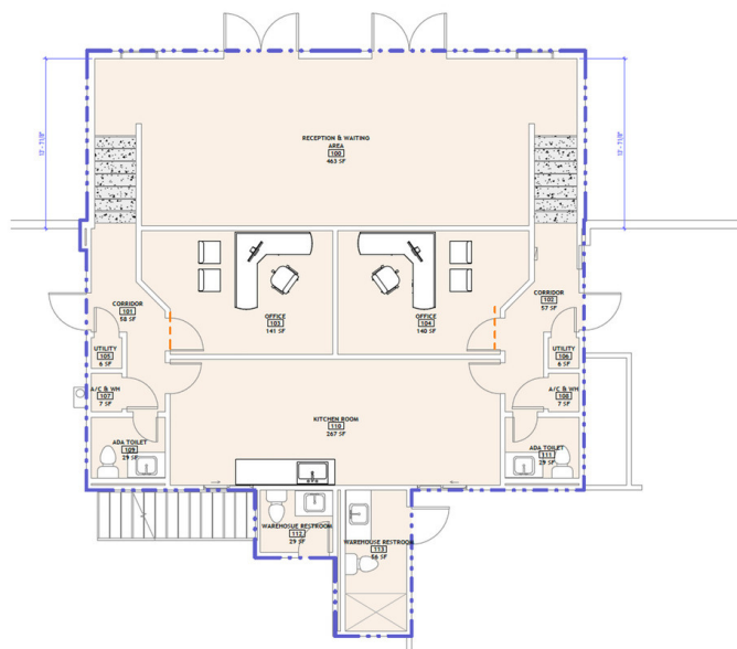
① FIRST FLOOR PLAN - OPTION 3 1/4" = 1'-0"
