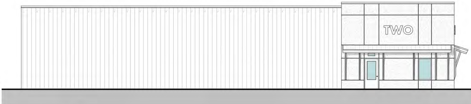
2 FRONT EXTERIOR ELEVATION - MKTG 3/16" = 1'-0"
