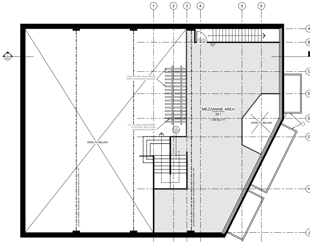
Bounce House Mezzanine Level Floor Plan 1 1/4" = 1'-0"
