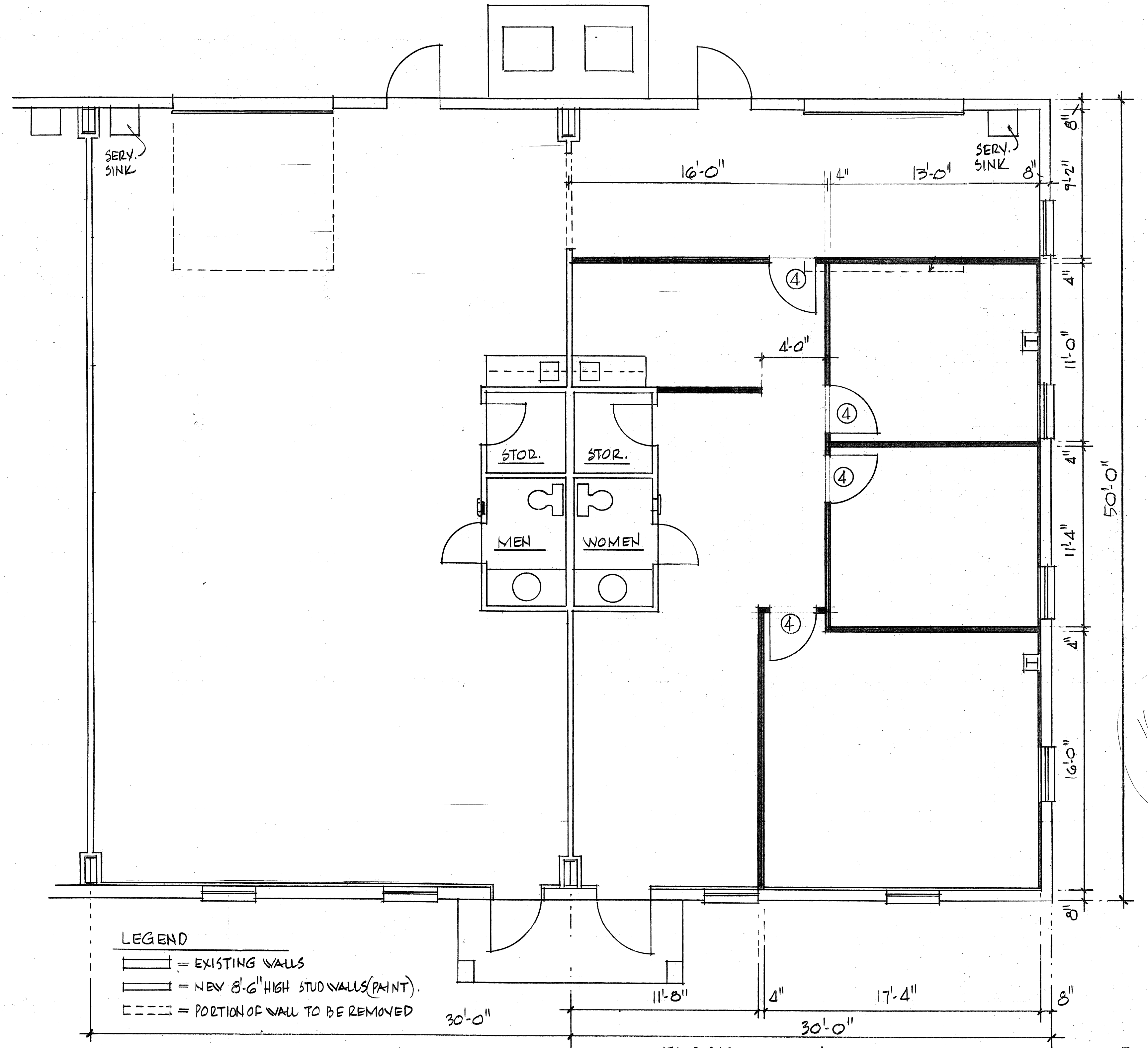
FLOOR PLAN 1/8"=1'-0"
