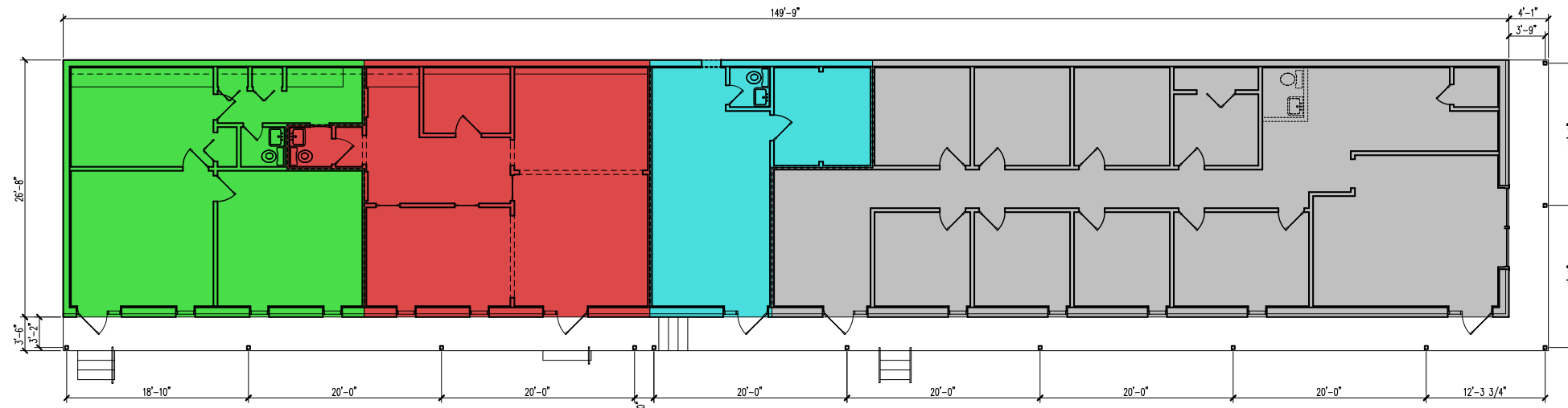
1 MAIN LEVEL - SINGLE STORY BUILDING AREA: 3,993.3 S.F.
