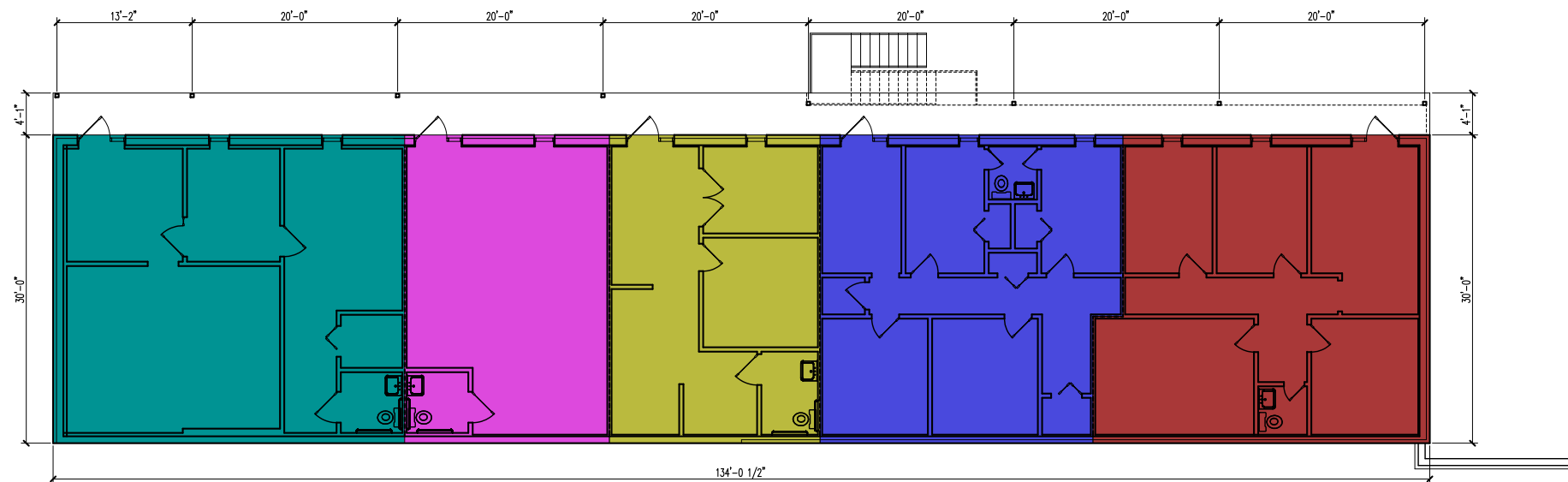
1 MAIN LEVEL - SINGLE STORY BUILDING AREA: 3,993.3 S.F.
