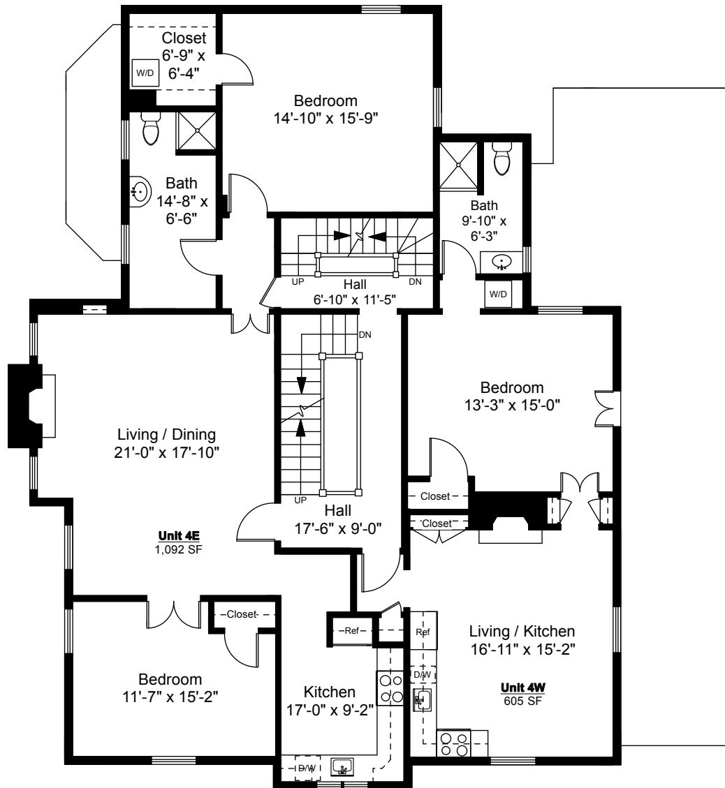
Second Floor Plan Ceiling Height = 10'-0"
