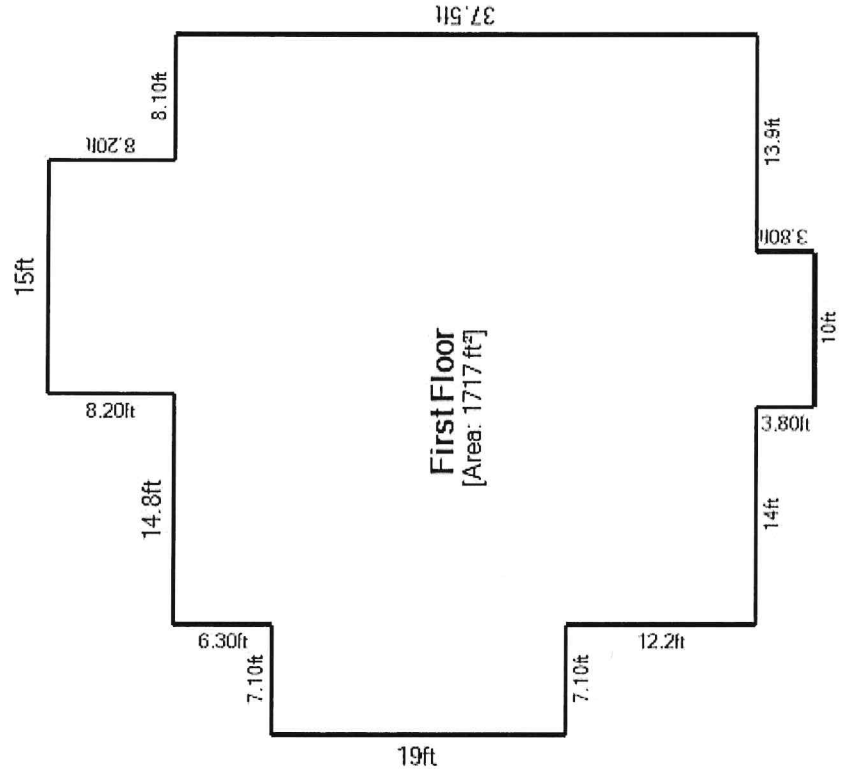
Building Footprint
