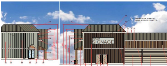
4 PROPOSED SIDE ELEVATION (CEDAR ST) SCALE: 1/8"=1'-0"
