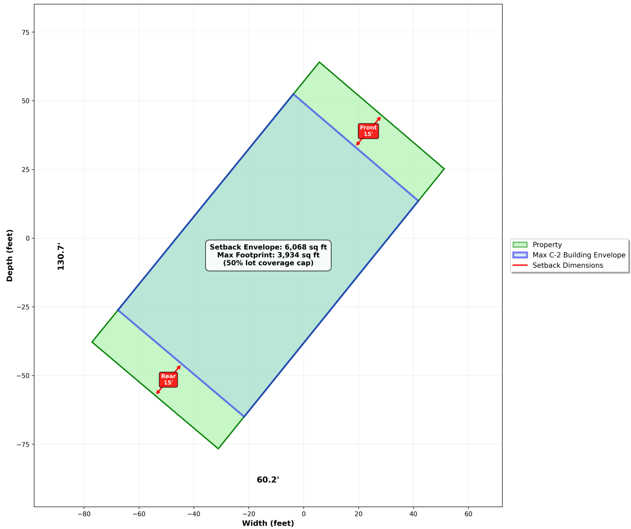
C-2 Zoning Site Plan - Parcel 6388004002 Lot Size: 60.2' x 130.7' (7,868 sq ft)
